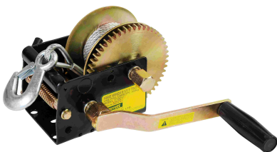
Model. F10217 HAND WINCH 5:1 / 1:1 (TWO RATIO) LINE PULL CAPACITY : 700KG
