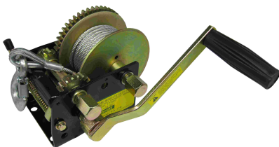
Model. F10950 HAND WINCH 10:1 / 5:1 / 1:1 (THREE RATIO) LINE PULL CAPACITY : 800KG
